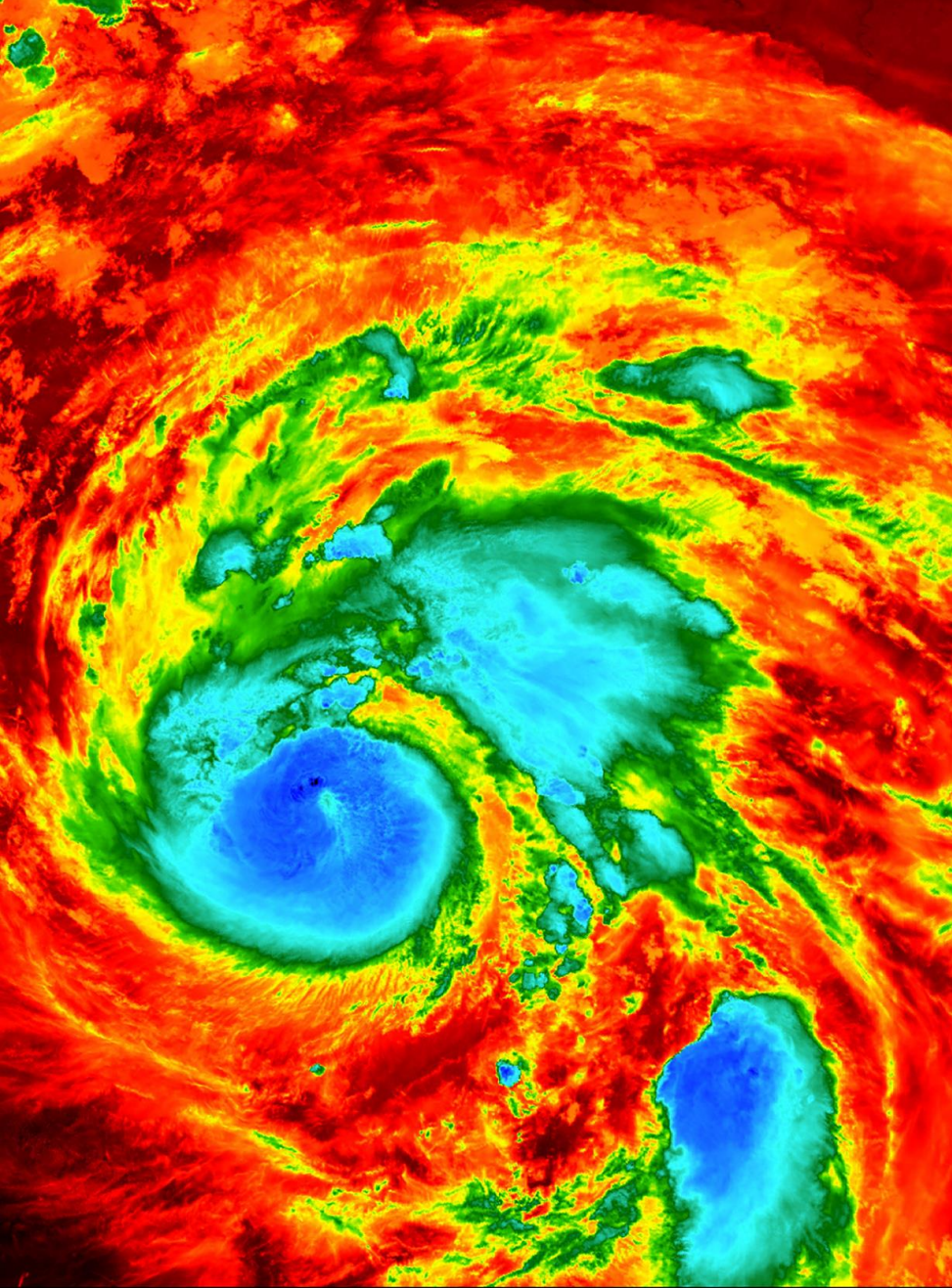
-60 -80 Top of atmosphere brightness temperature (°C)
